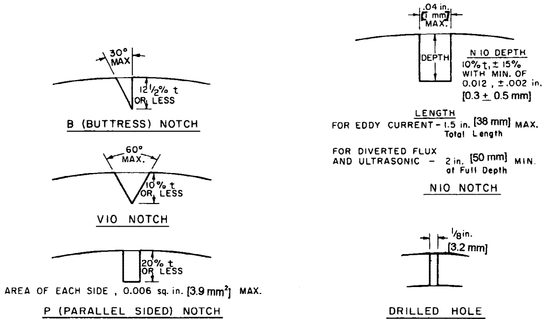
FIG. 1 Calibration Standards
